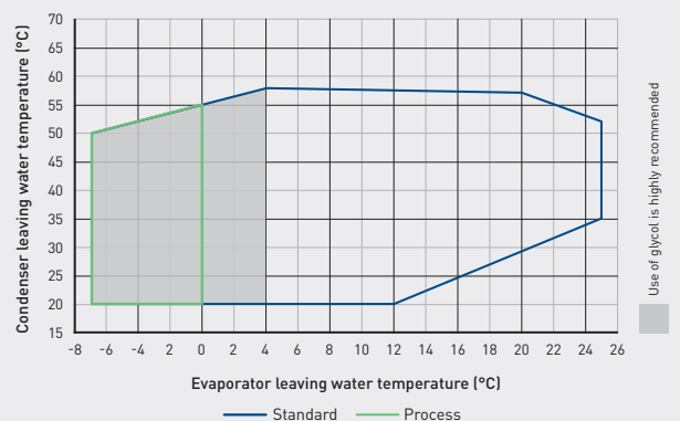
NEPTUNE G HP GEO | Operating limits
